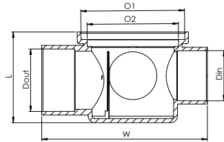
Floor Drain 110/125 with Odor Trap
