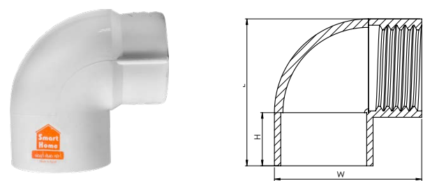
Elbow 87.5° with inner thread
