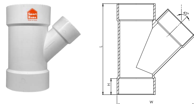
Tee 45° Reducer
