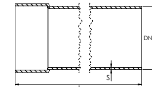
Multi Layer PiPeS with solvent cement socket
