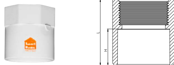
Socket with Inner Thread
