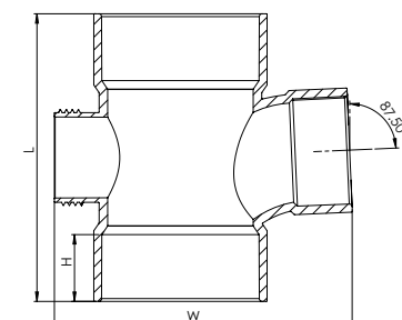
Tee 87.5° Reducer with Access Door Reducer
