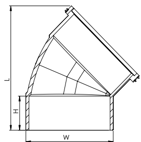
Elbow 45° with expansion Joint
